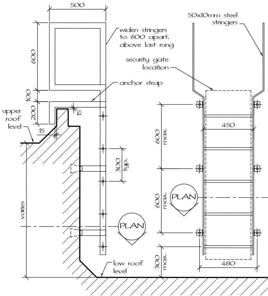
SECTION
