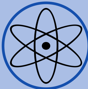
PHYSICS
