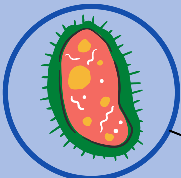
BIOLOGY
