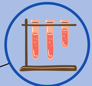
CHEMISTRY
